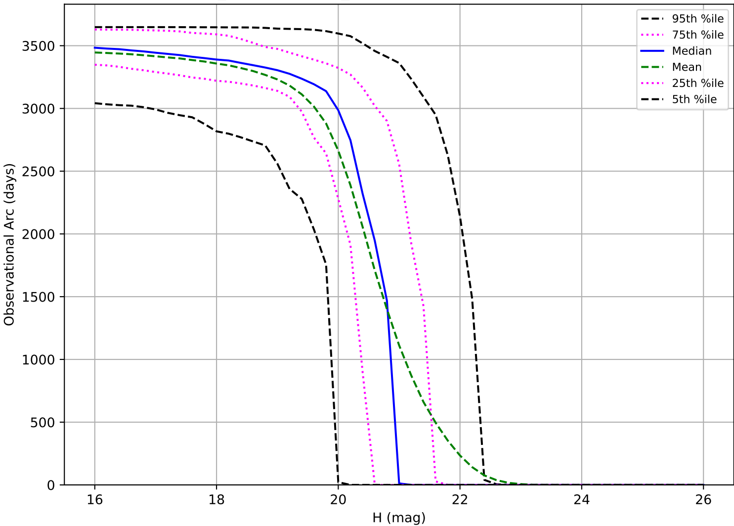
weather_cloudso20v3.4_10yrs: Observational Arc Length MBA
