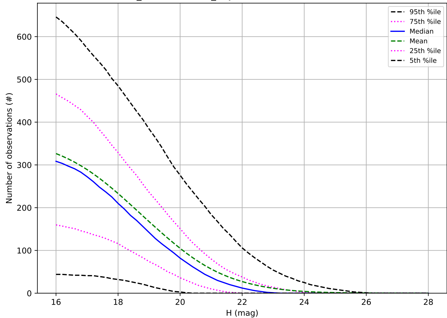
weather_cloudso20v3.4_10yrs: Number of observations PHA
