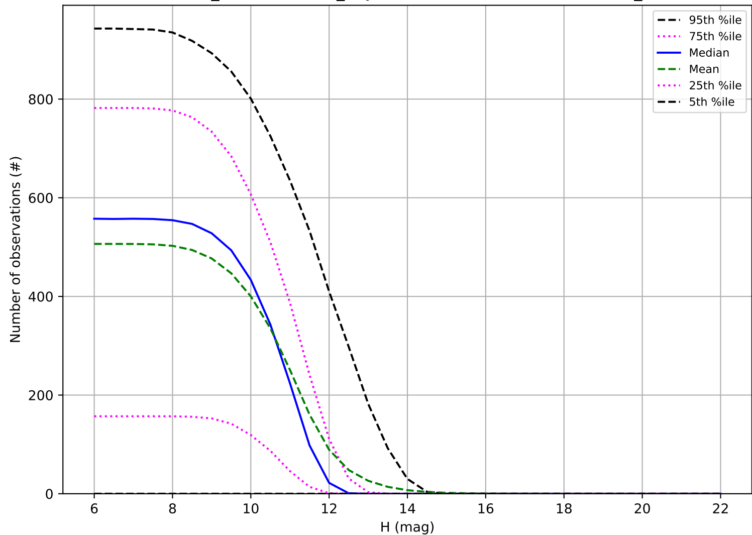
weather_cloudso20v3.4_10yrs: Number of observations OCC_r20
