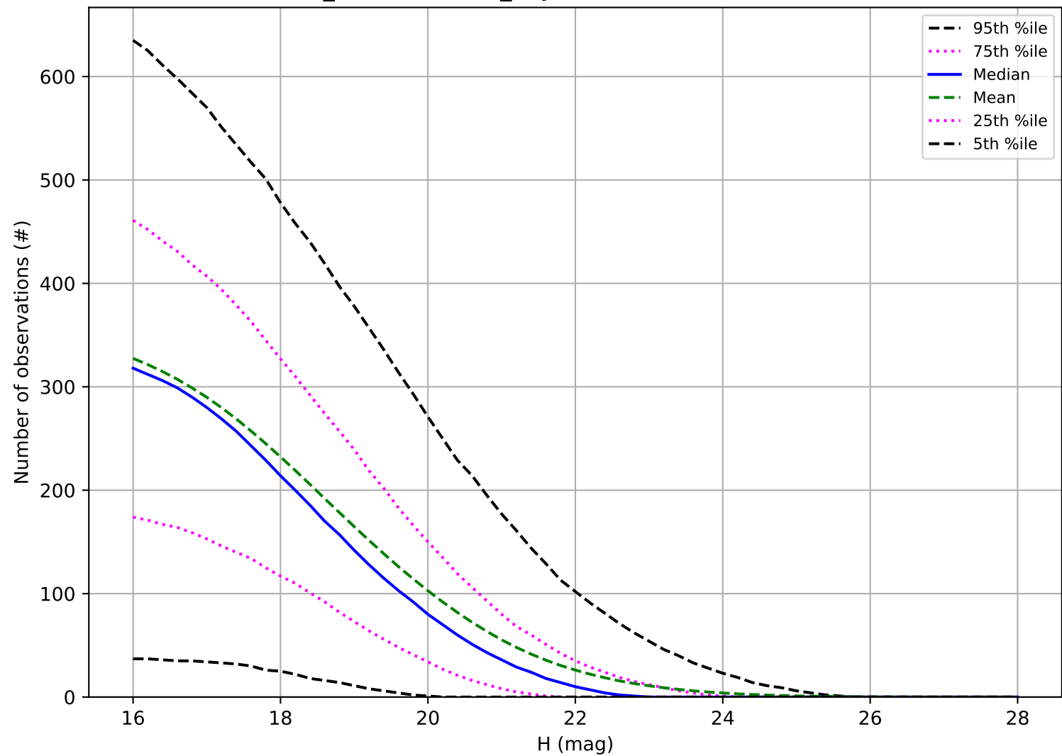
weather_cloudso20v3.4_10yrs: Number of observations NEO
