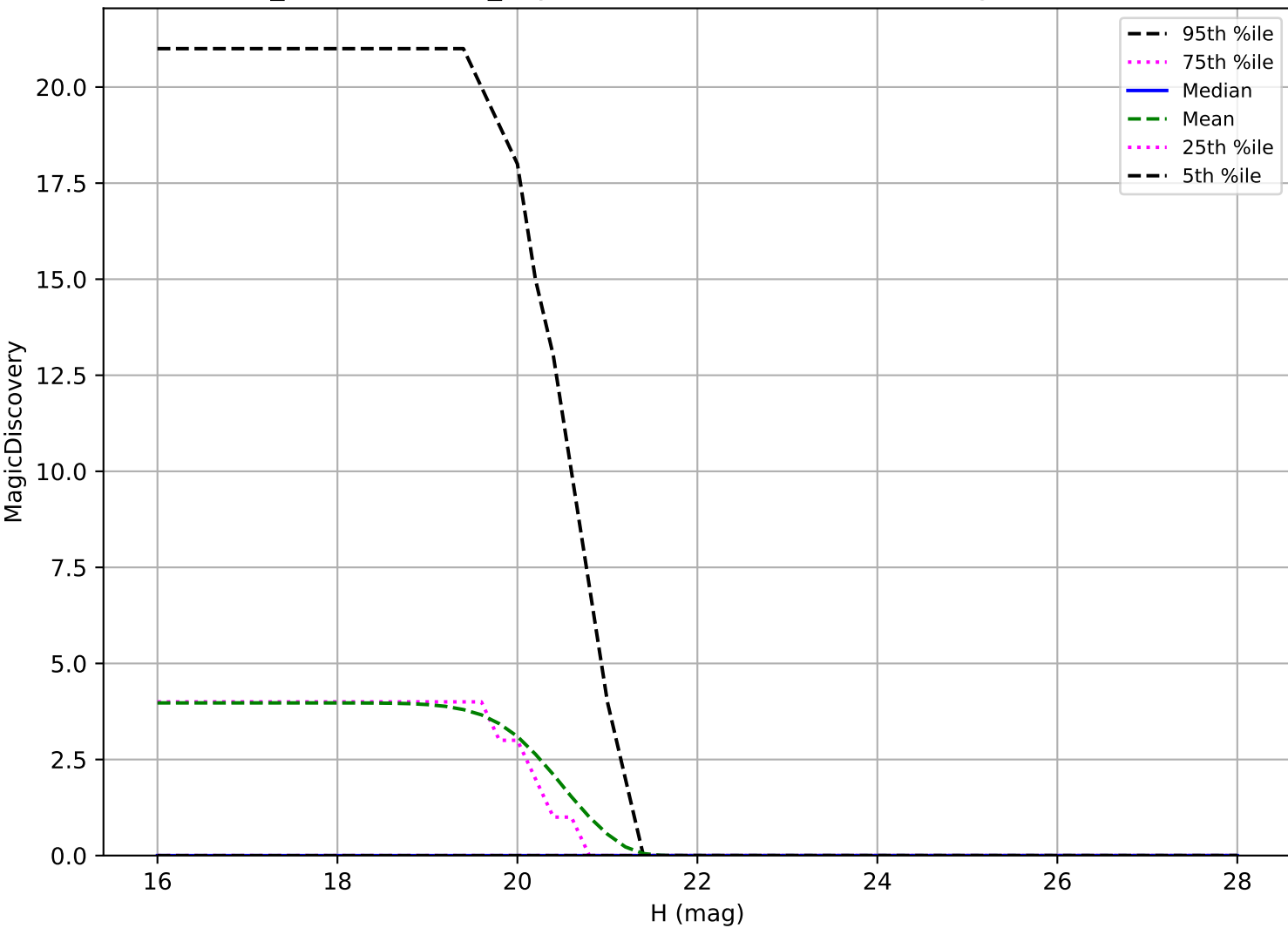
weather_cloudso20v3.4_10yrs: Vatira 6 detections in 60 nights detection loss
