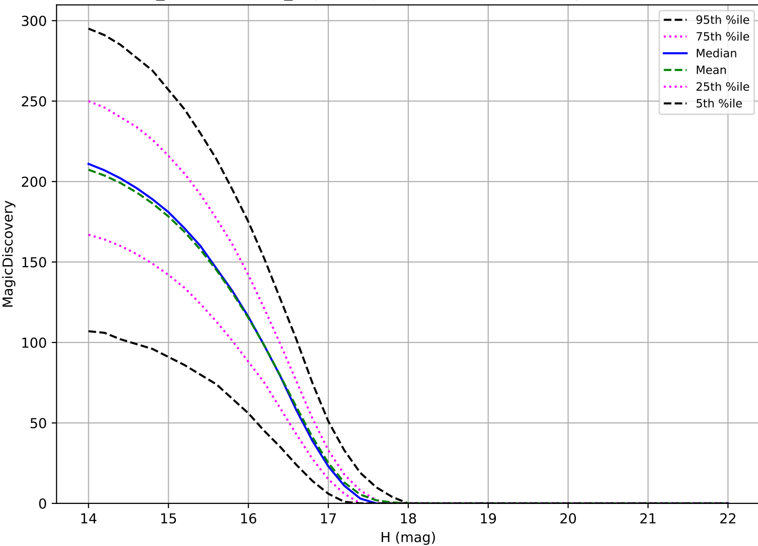
weather_cloudso20v3.4_10yrs: Trojan 6 detections in 60 nights detection loss
