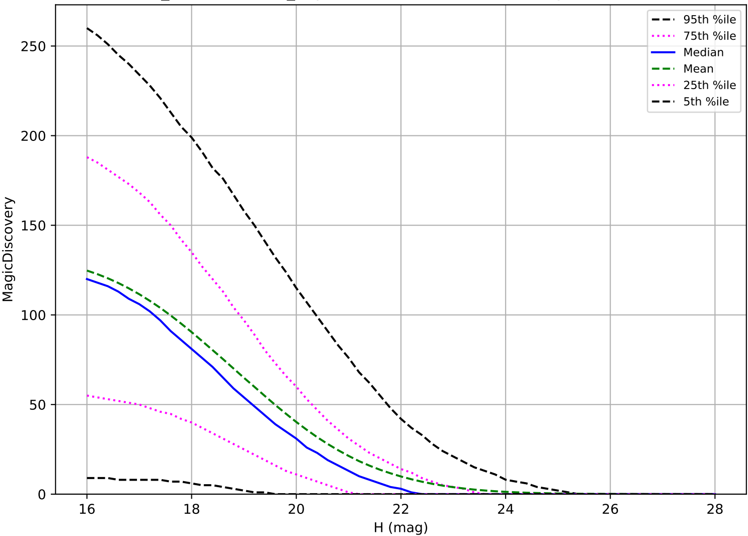
weather_cloudso20v3.4_10yrs: PHA 6 detections in 60 nights detection loss
