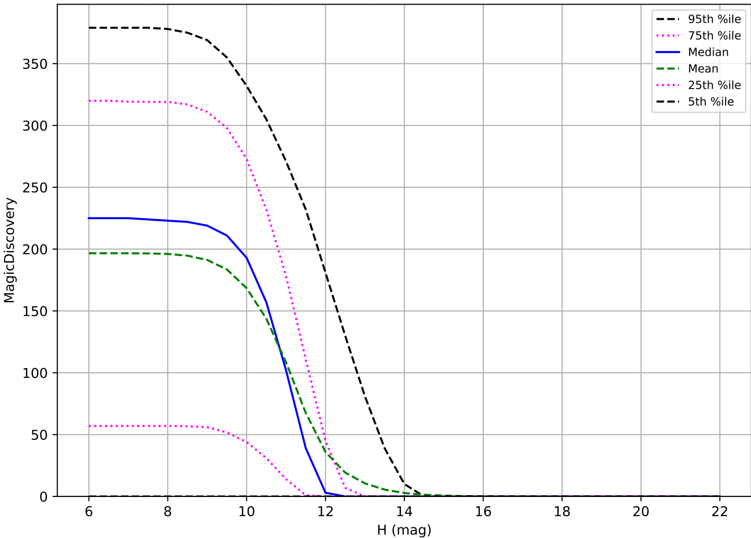
weather_cloudso20v3.4_10yrs: OCC_r20 6 detections in 60 nights detection loss
