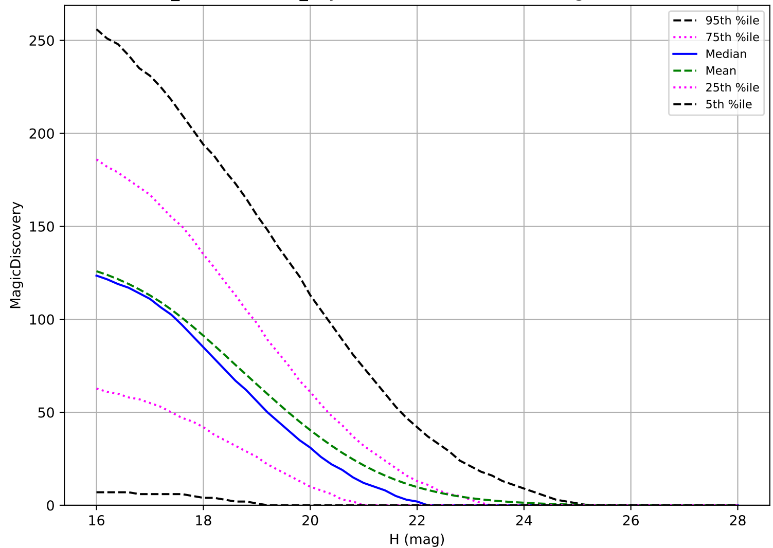
weather_cloudso20v3.4_10yrs: NEO 6 detections in 60 nights detection loss
