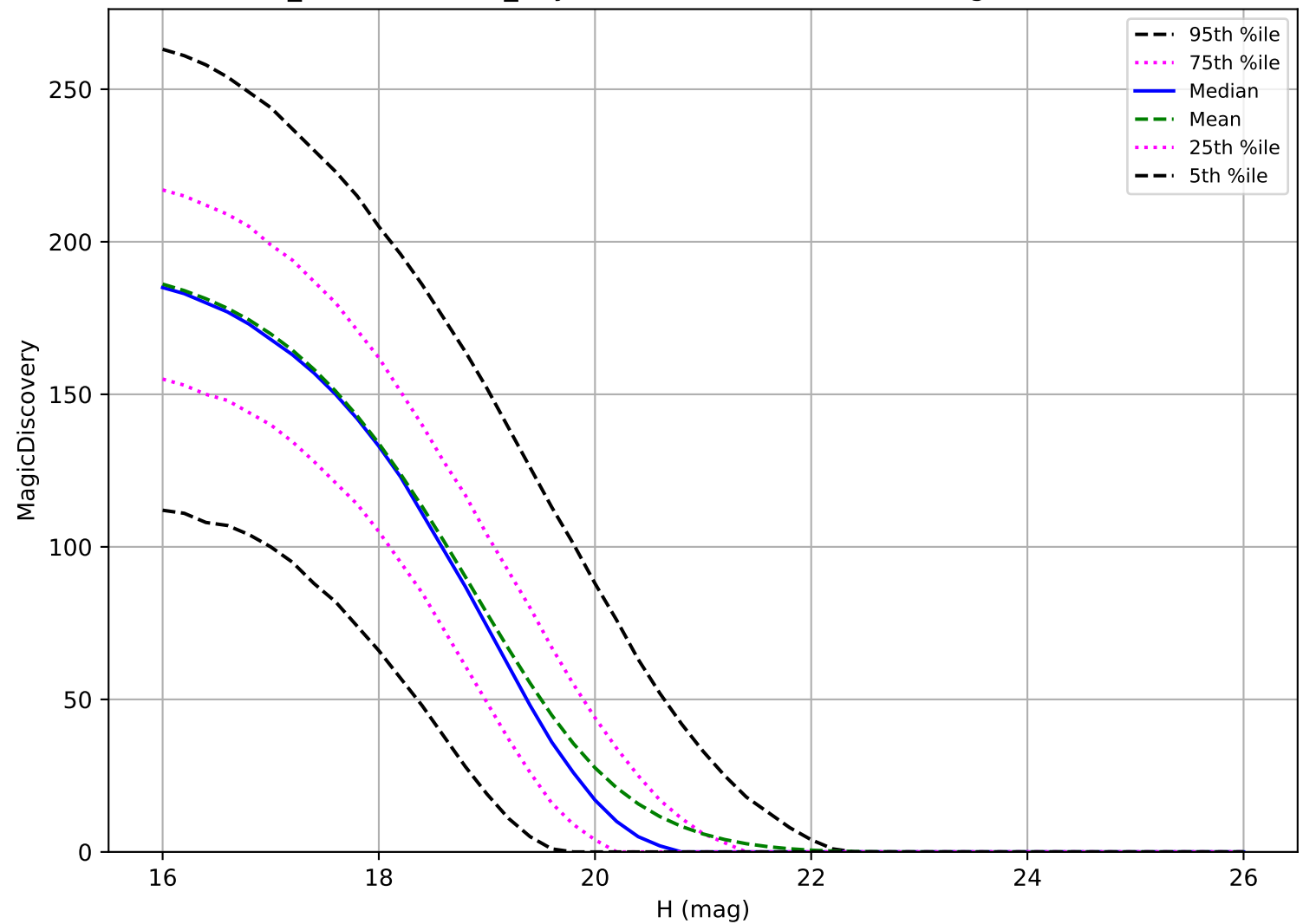
weather_cloudso20v3.4_10yrs: MBA 6 detections in 60 nights detection loss
