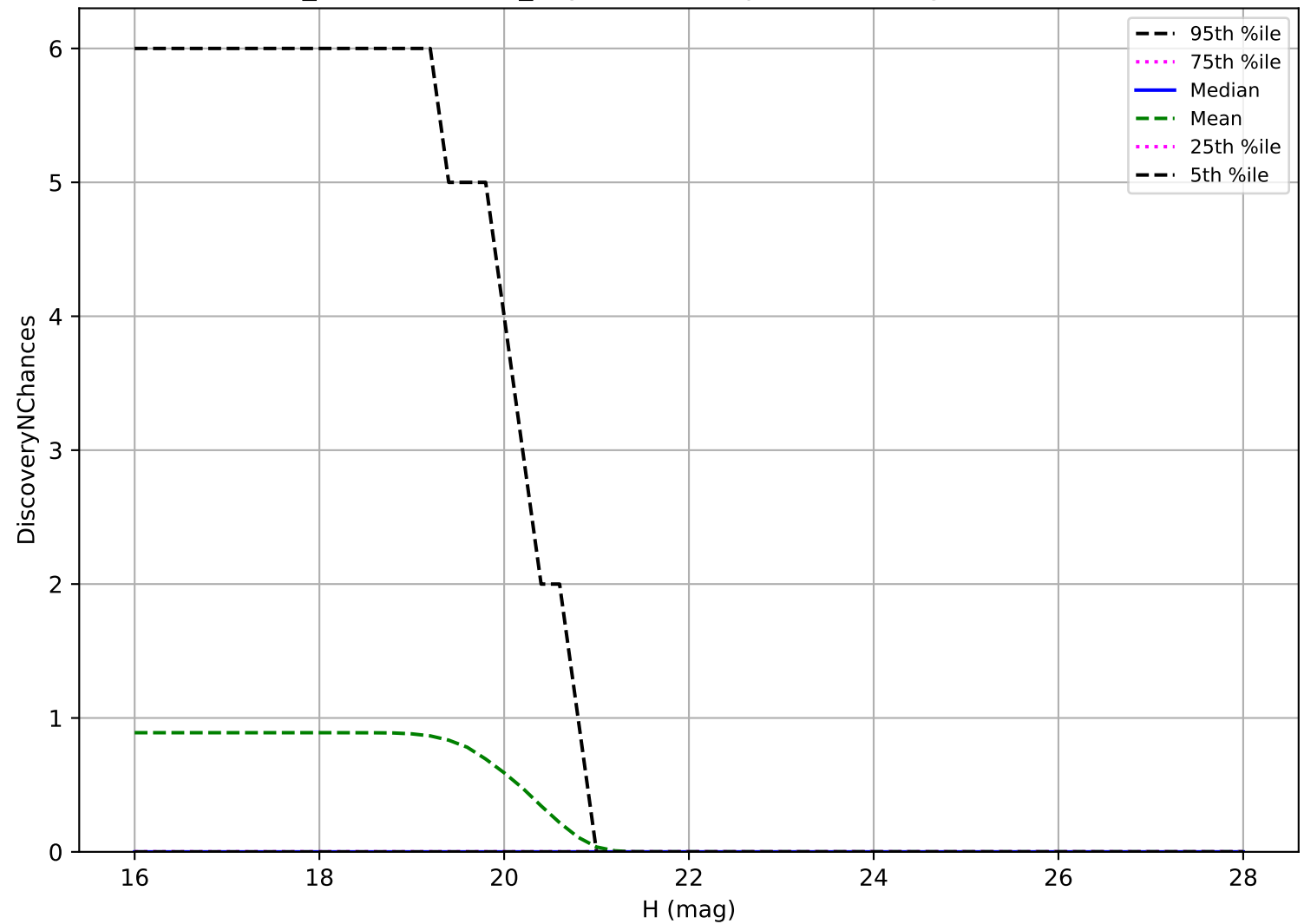
weather_cloudso20v3.4_10yrs: Vatira 3 pairs in 15 nights detection loss
