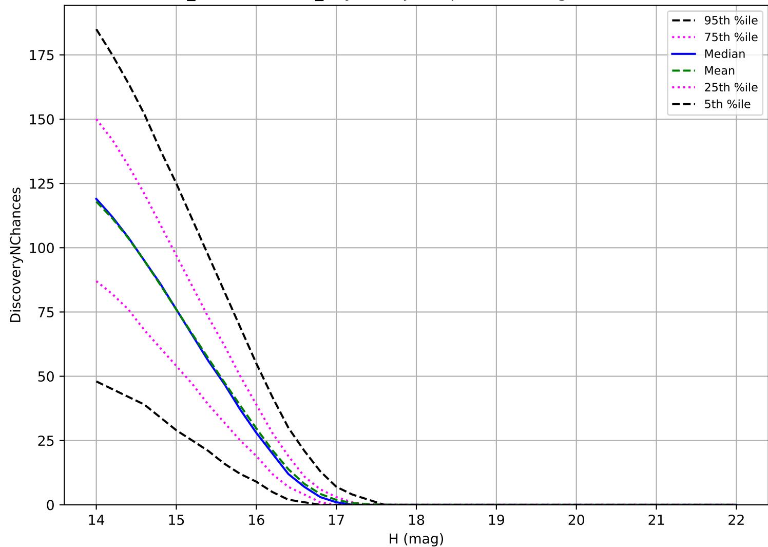
weather_cloudso20v3.4_10yrs: Trojan 3 pairs in 15 nights detection loss
