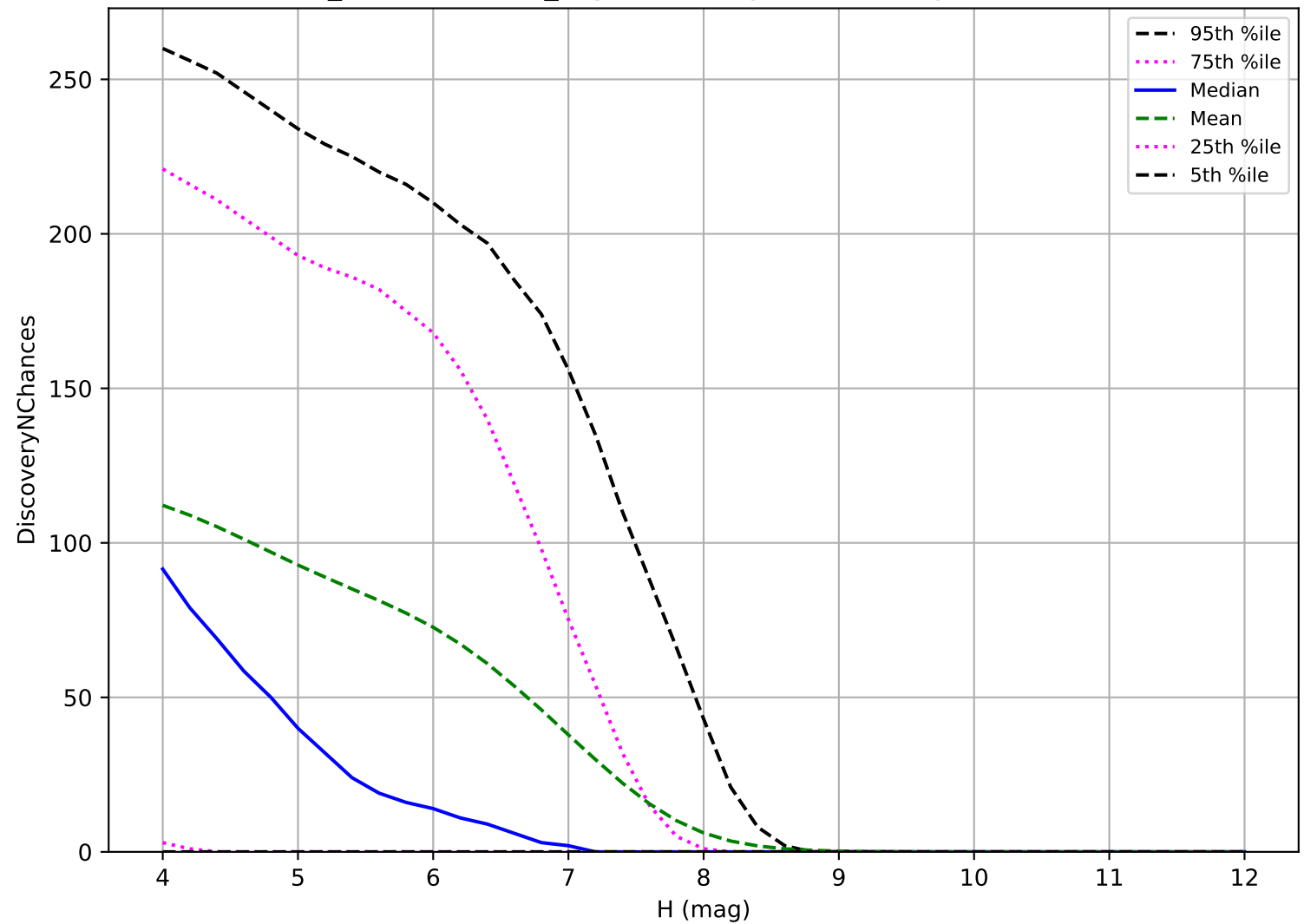
weather_cloudso20v3.4_10yrs: TNO 3 pairs in 15 nights detection loss
