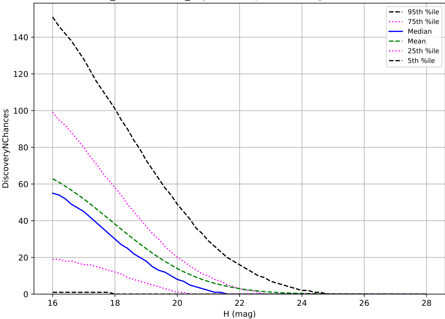
weather_cloudso20v3.4_10yrs: PHA 3 pairs in 15 nights detection loss
