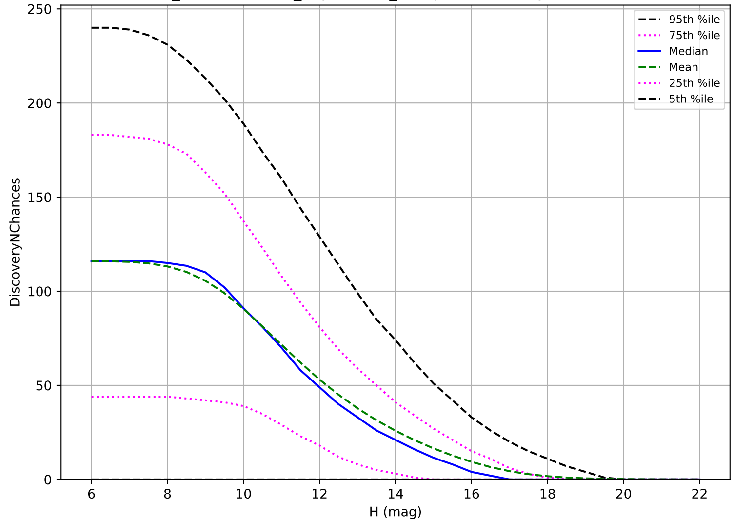
weather_cloudso20v3.4_10yrs: OCC_r5 3 pairs in 15 nights detection loss
