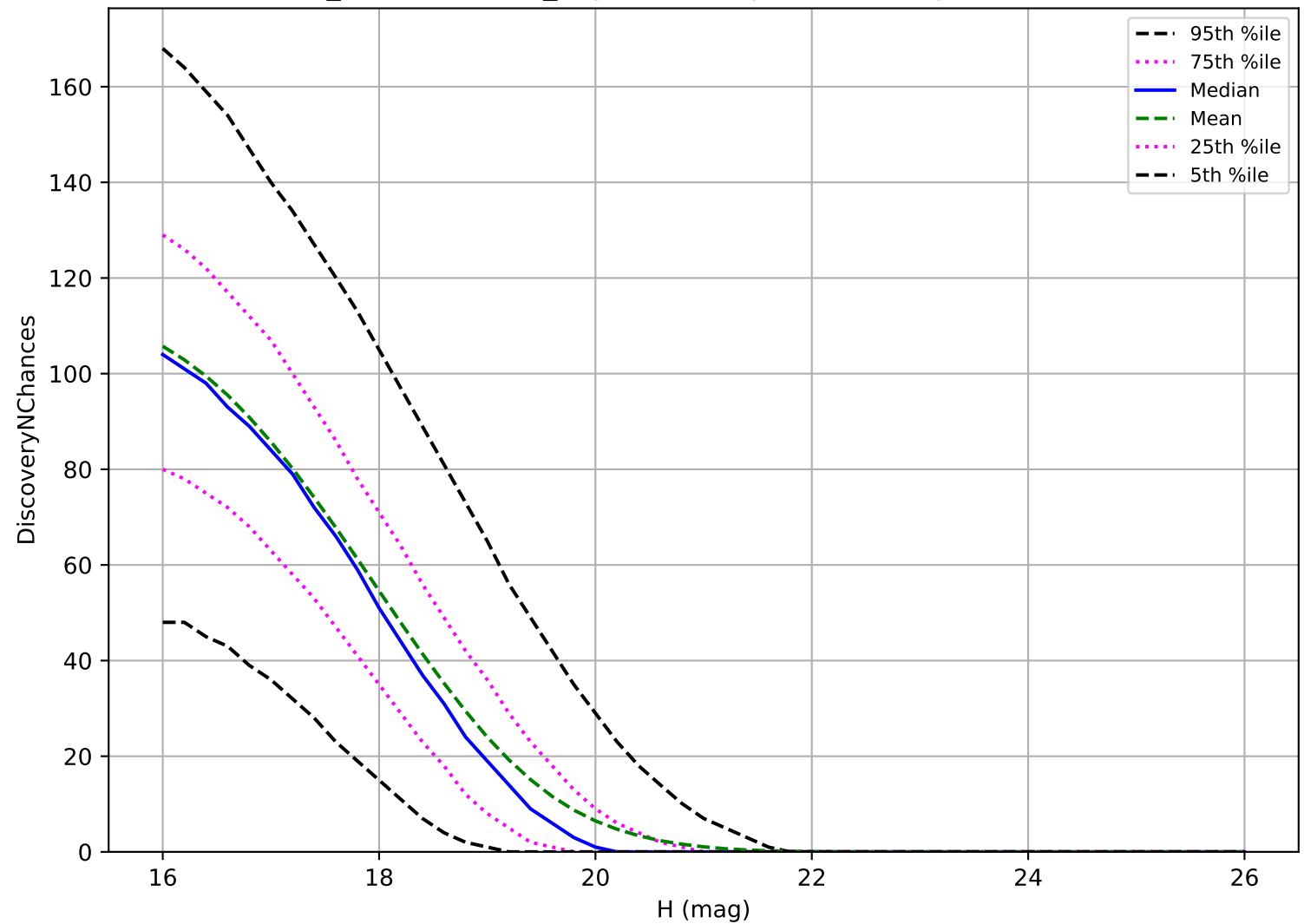
weather_cloudso20v3.4_10yrs: MBA 3 pairs in 15 nights detection loss
