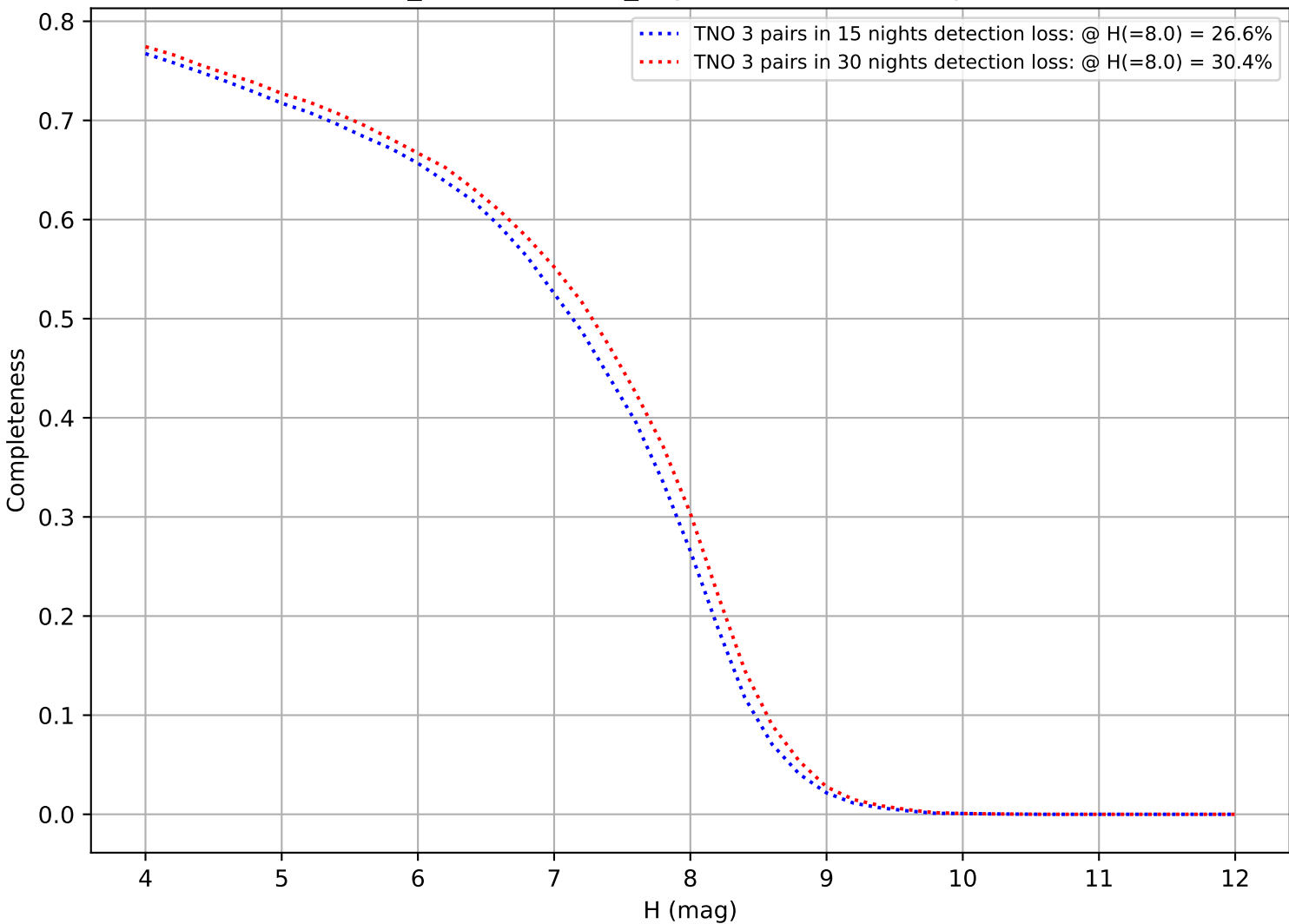
weather_cloudso20v3.4_10yrs: DifferentialCompleteness
