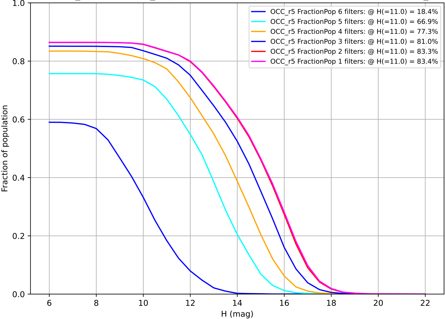
weather_cloudso20v3.4_10yrs: Fraction of population with colors in X filters OCC_r5
