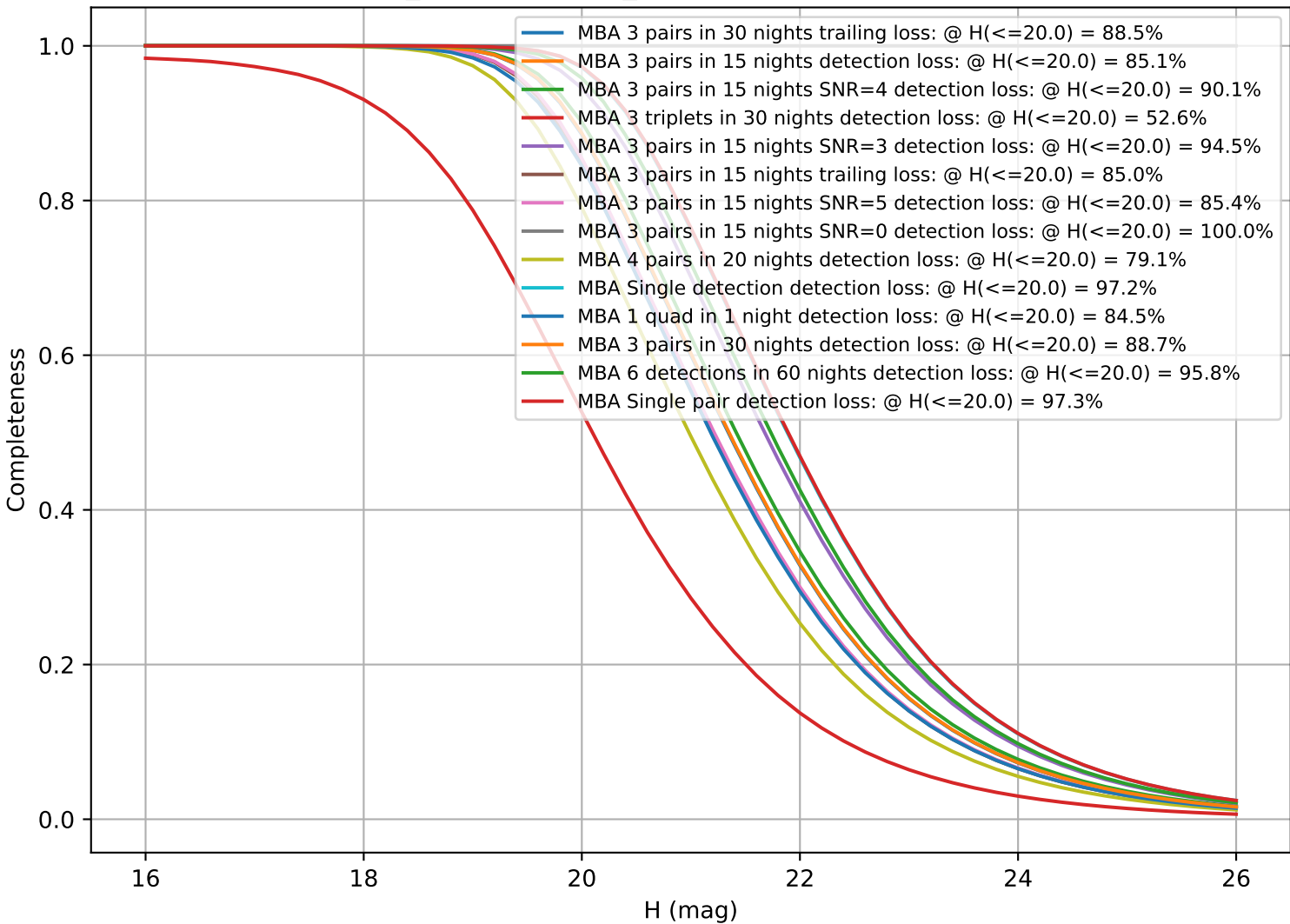
weather_cloudso20v3.4_10yrs: CumulativeCompleteness
