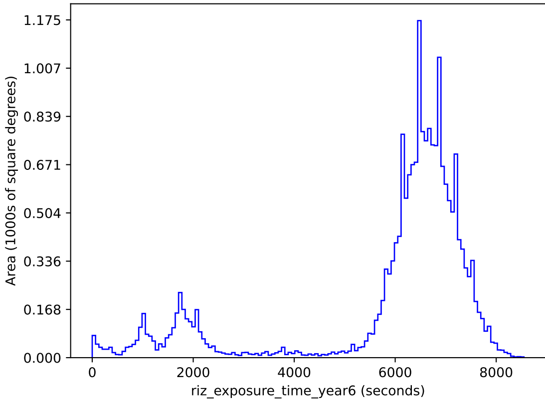
weather_cloudso20v3.4_10yrs gri band non-DD: riz_exposure_time_year6
