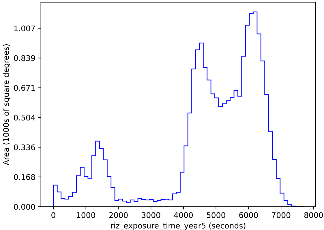
weather_cloudso20v3.4_10yrs gri band non-DD: riz_exposure_time_year5
