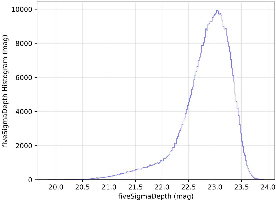
weather_cloudso20v3.4_10yrs z: fiveSigmaDepth Histogram
