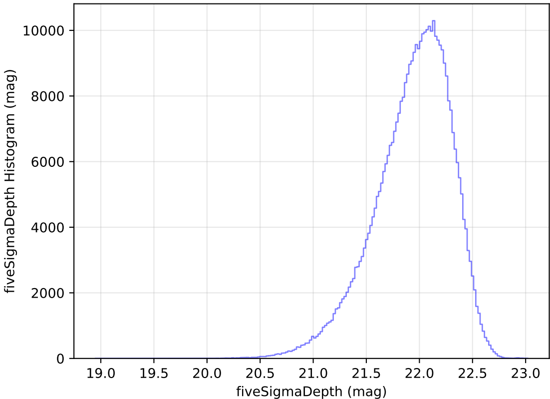
weather_cloudso20v3.4_10yrs y: fiveSigmaDepth Histogram
