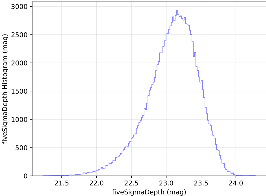
weather_cloudso20v3.4_10yrs u: fiveSigmaDepth Histogram
