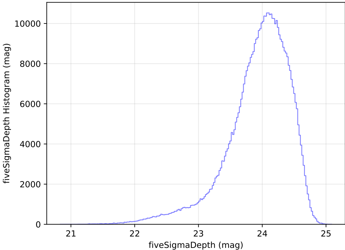
weather_cloudso20v3.4_10yrs r: fiveSigmaDepth Histogram
