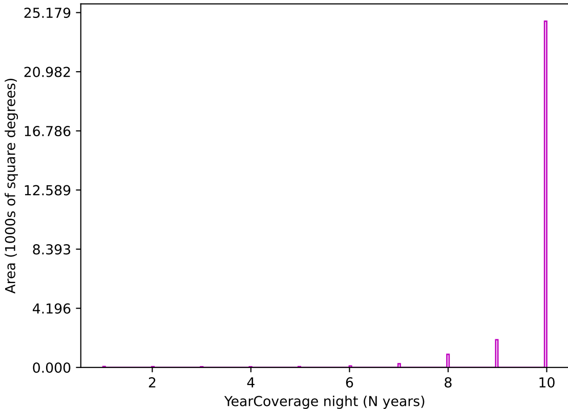
weather_cloudso20v3.4_10yrs z band: YearCoverage night
