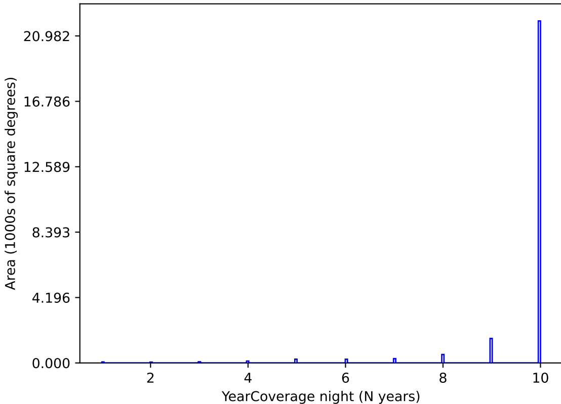
weather_cloudso20v3.4_10yrs y band: YearCoverage night
