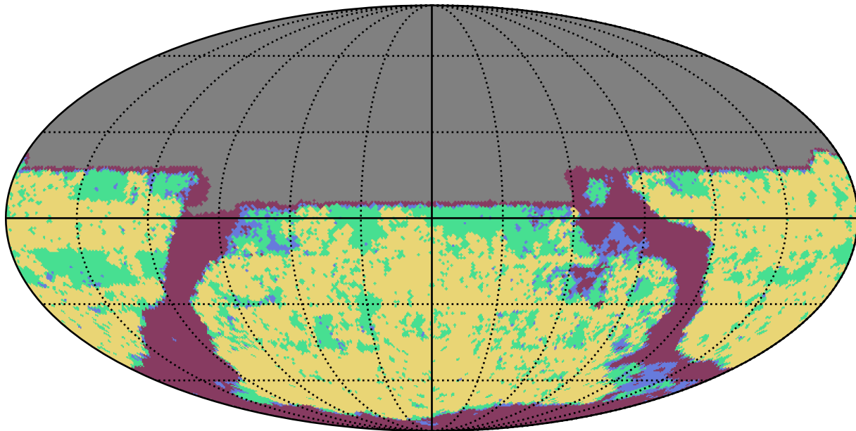
weather_cloudso20v3.4_10yrs u band: YearCoverage night
