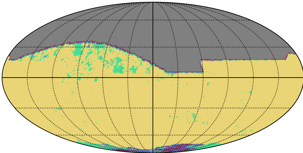
weather_cloudso20v3.4_10yrs r band: YearCoverage night
