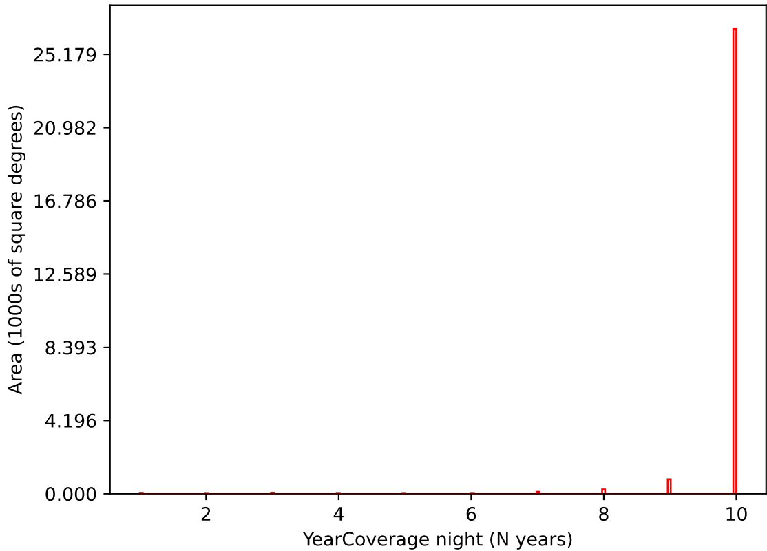
weather_cloudso20v3.4_10yrs i band: YearCoverage night
