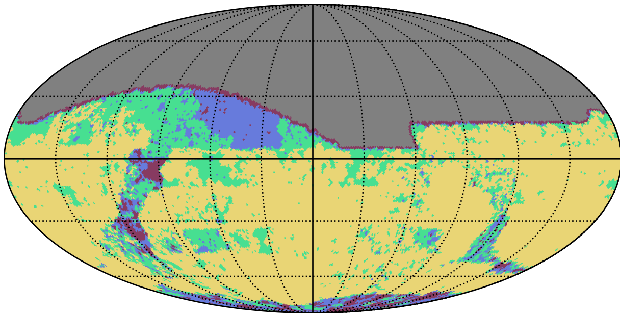
weather_cloudso20v3.4_10yrs g band: YearCoverage night
