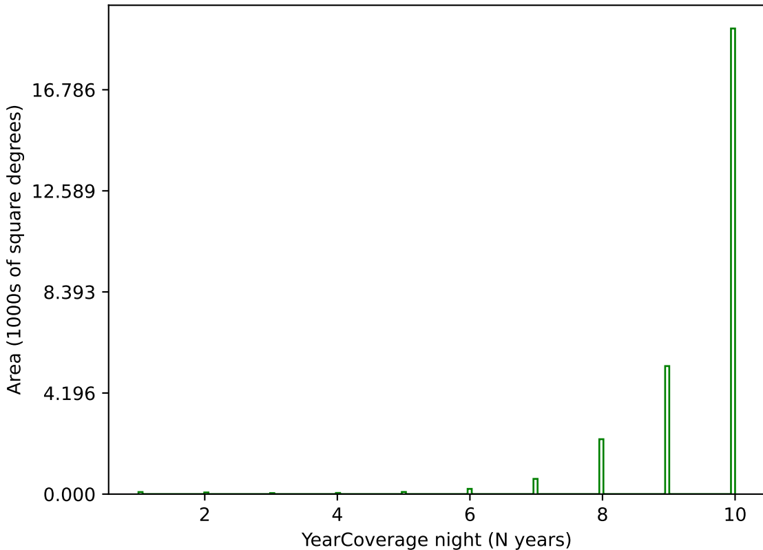
weather_cloudso20v3.4_10yrs g band: YearCoverage night
