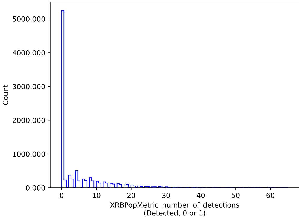
weather_cloudso20v3.4_10yrs : XRBPoMetric_number_of_detections
