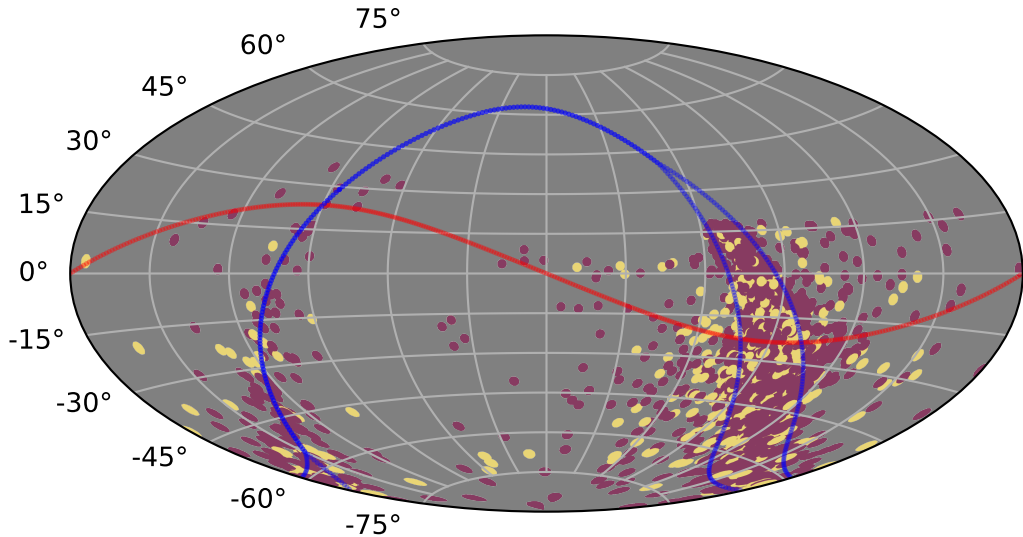
weather_cloudso20v3.4_10yrs : XRBPopMetric_early_detect
