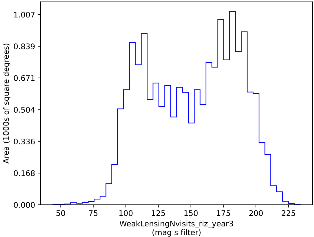
weather_cloudso20v3.4_10yrs gri band non-DD: WeakLensingNvisits_riz_year3
