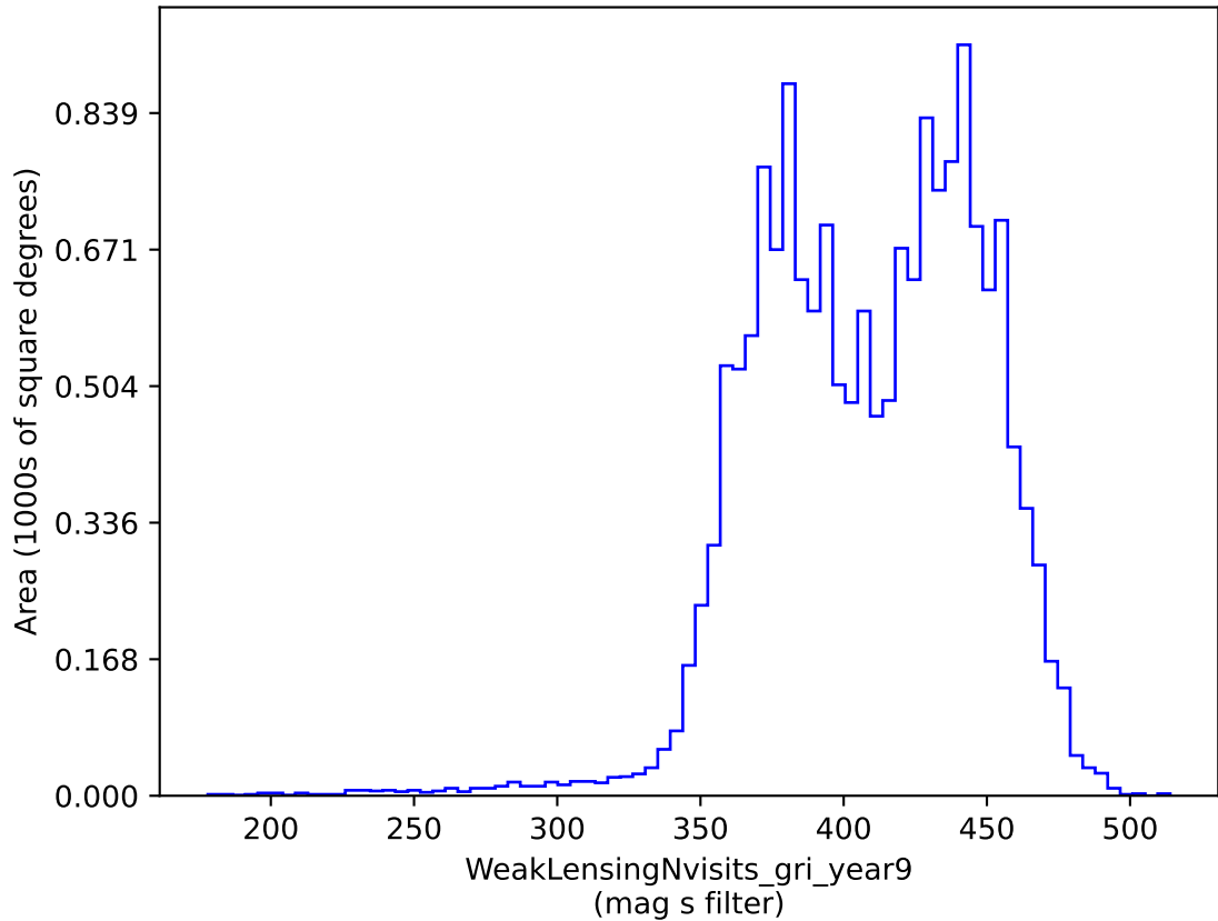
weather_cloudso20v3.4_10yrs gri band non-DD: WeakLensingNvisits_gri_year9
