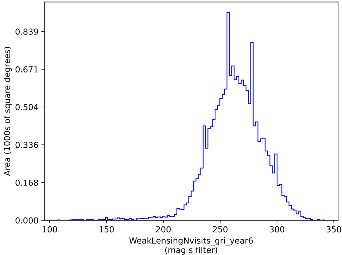
weather_cloudso20v3.4_10yrs gri band non-DD: WeakLensingNvisits_gri_year6
