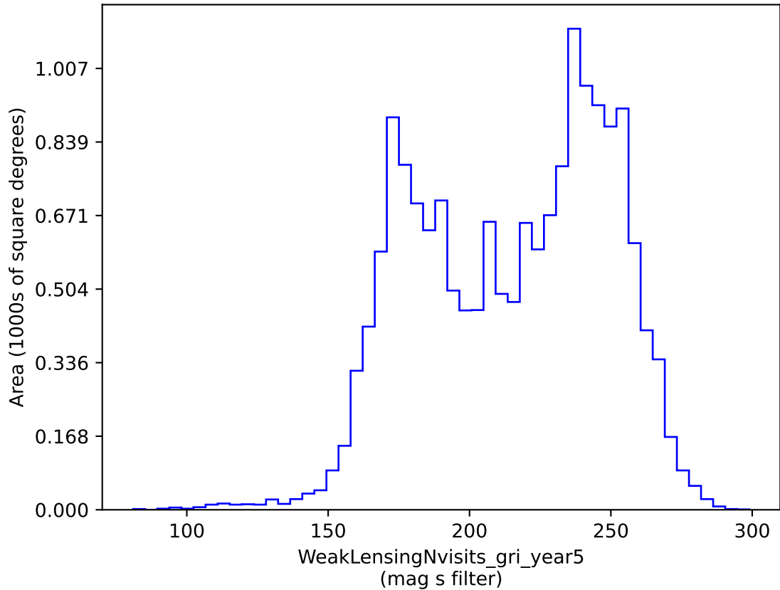
weather_cloudso20v3.4_10yrs gri band non-DD: WeakLensingNvisits_gri_year5
