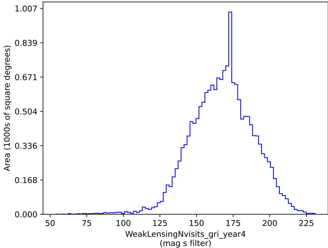
weather_cloudso20v3.4_10yrs gri band non-DD: WeakLensingNvisits_gri_year4
