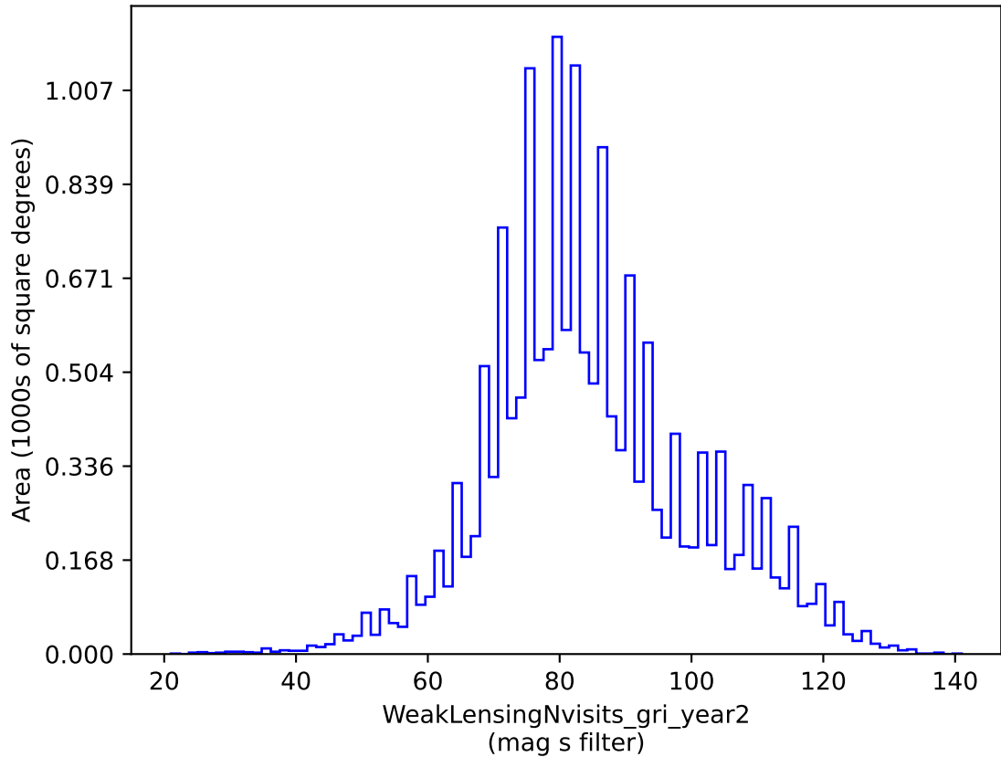
weather_cloudso20v3.4_10yrs gri band non-DD: WeakLensingNvisits_gri_year2
