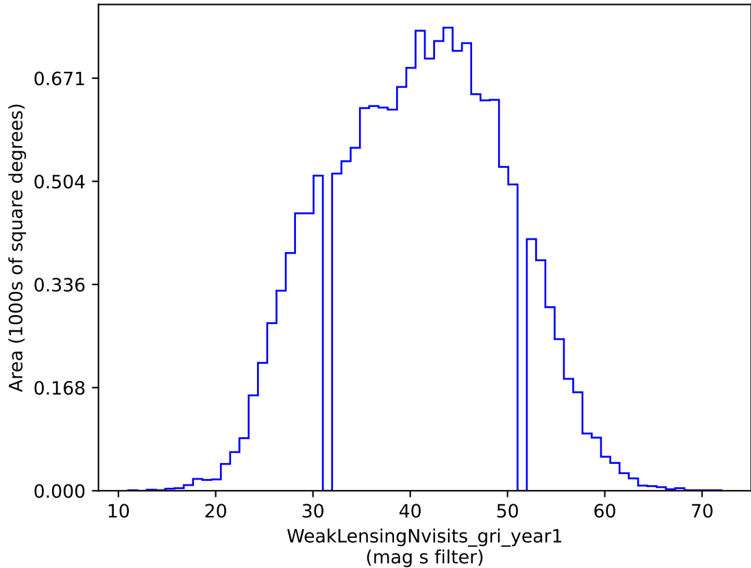
weather_cloudso20v3.4_10yrs gri band non-DD: WeakLensingNvisits_gri_year1
