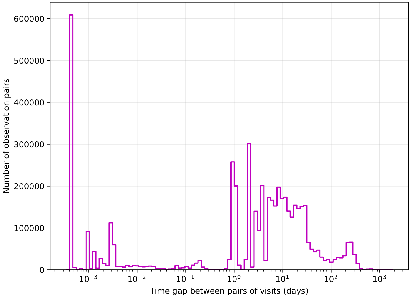
weather_cloudso20v3.4_10yrs z band: Tgaps observationStartMJD
