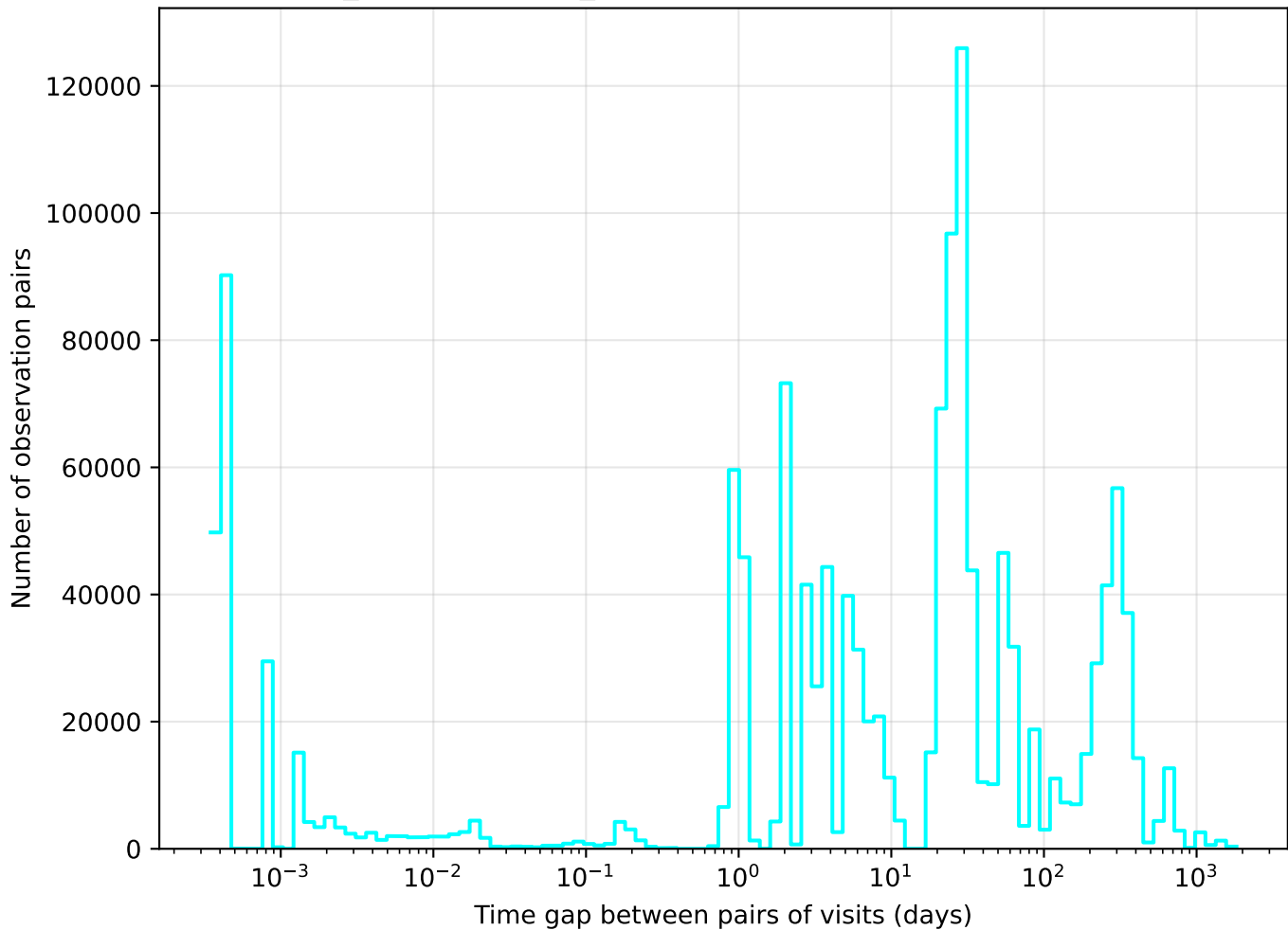
weather_cloudso20v3.4_10yrs u band: Tgaps observationStartMJD
