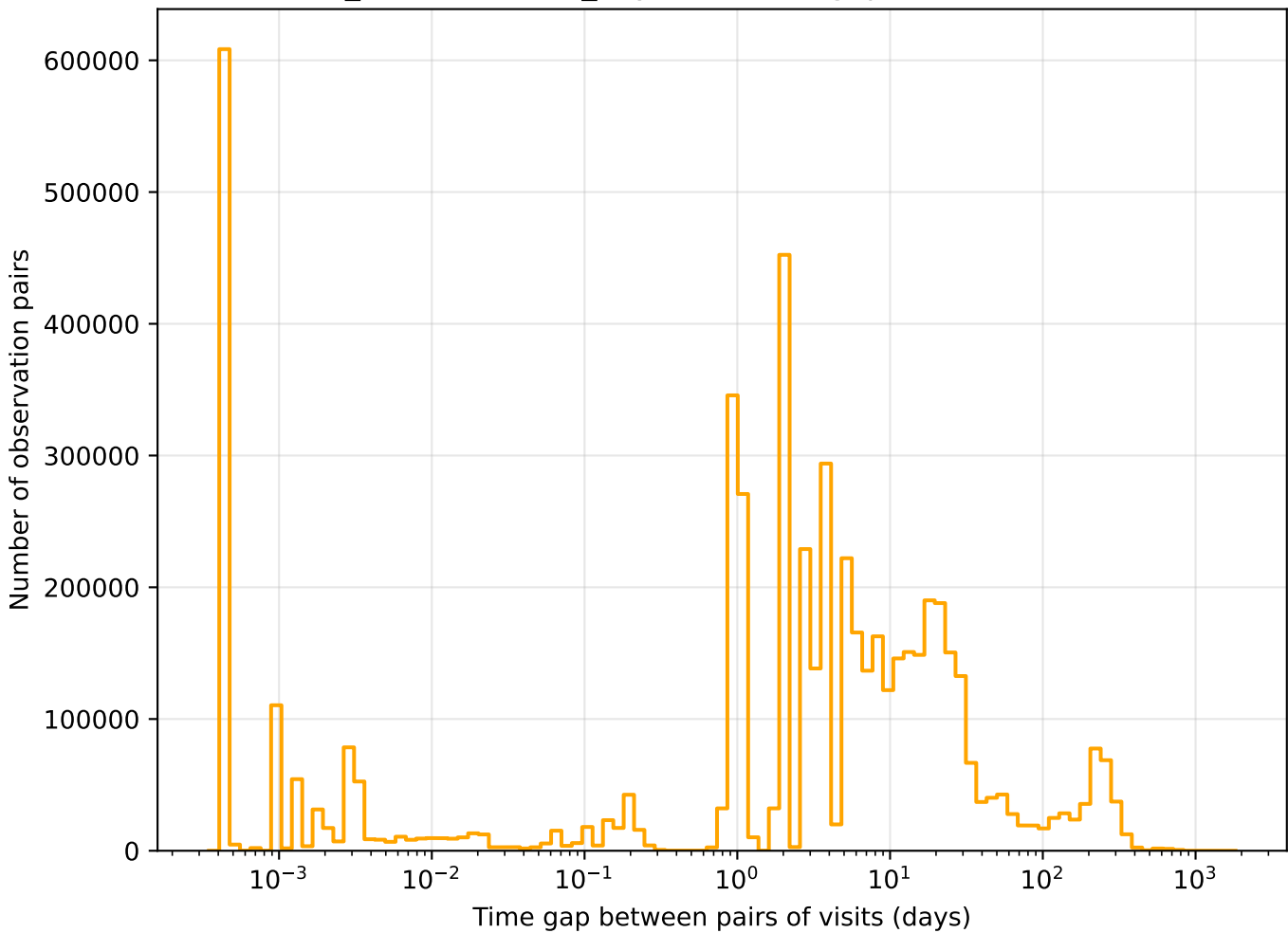
weather_cloudso20v3.4_10yrs r band: Tgaps observationStartMJD
