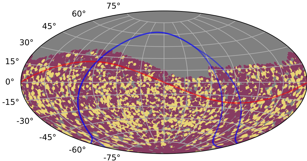
weather_cloudso20v3.4_10yrs : TDEsPopMetric_prepeak
