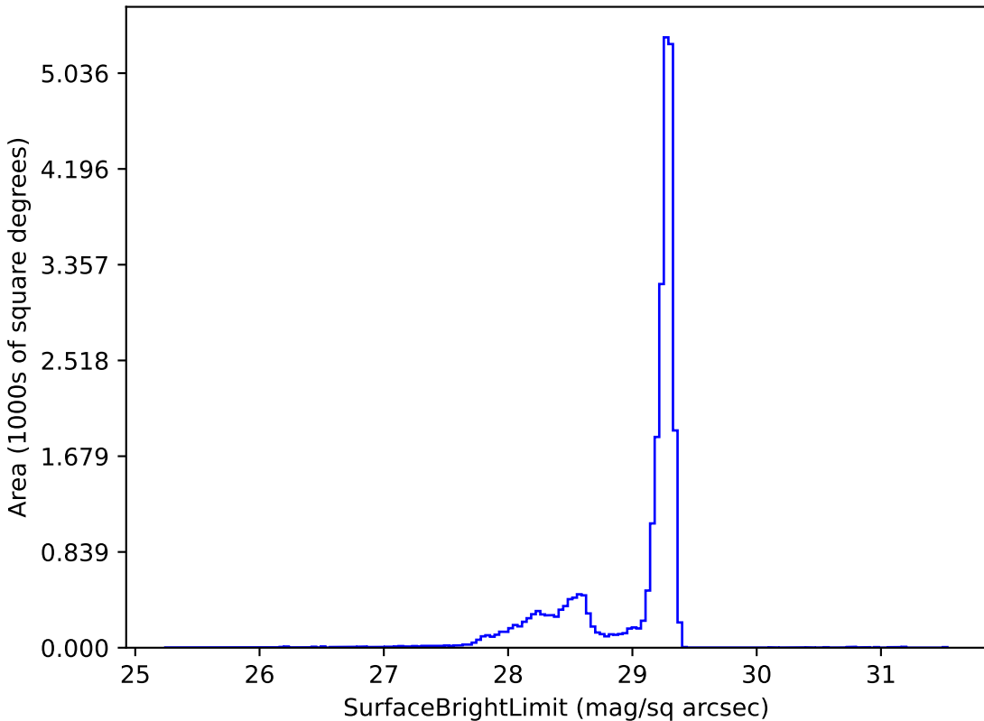
weather_cloudso20v3.4_10yrs z: SurfaceBrightLimit
