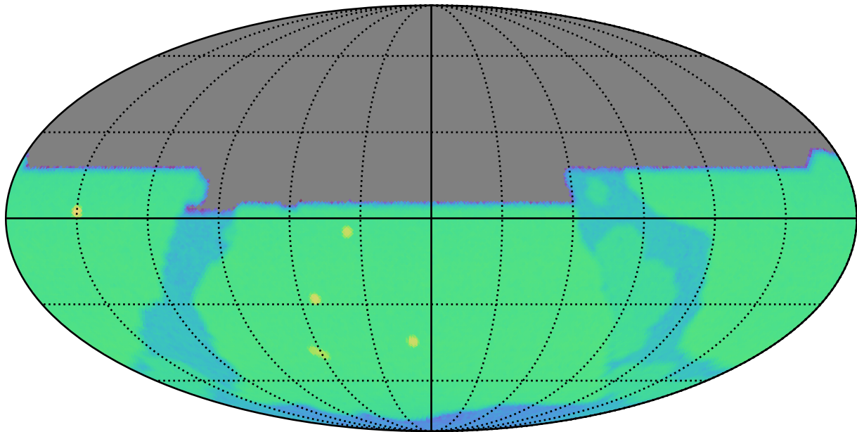
weather_cloudso20v3.4_10yrs y: SurfaceBrightLimit
