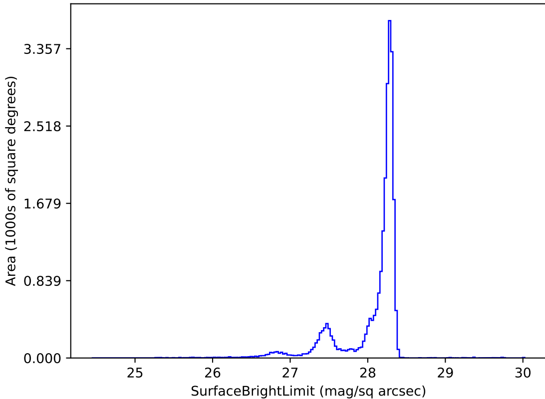
weather_cloudso20v3.4_10yrs y: SurfaceBrightLimit
