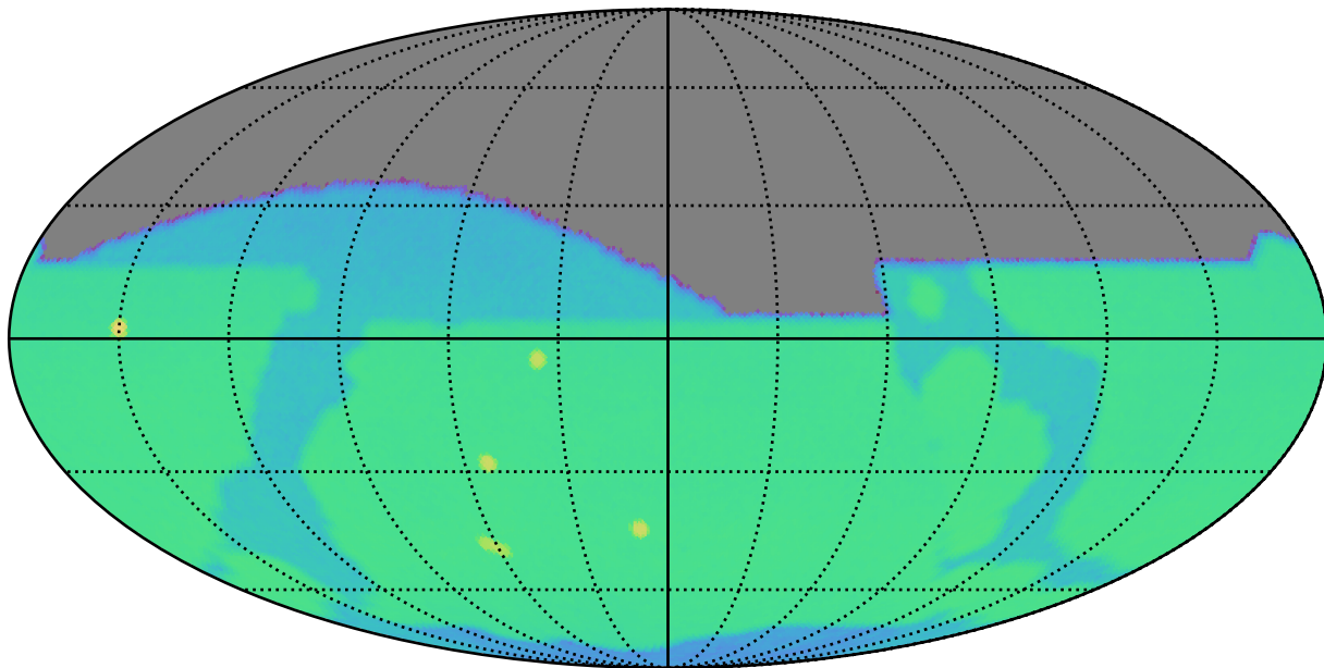
weather_cloudso20v3.4_10yrs r: SurfaceBrightLimit
