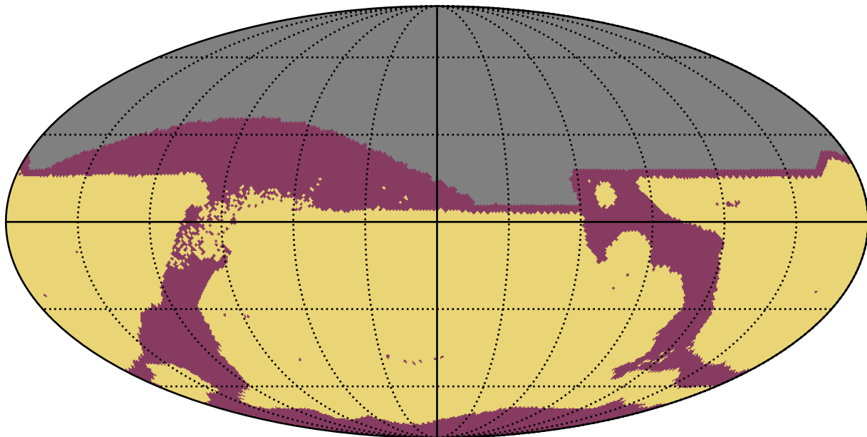
weather_cloudso20v3.4_10yrs : RapidRevisits
